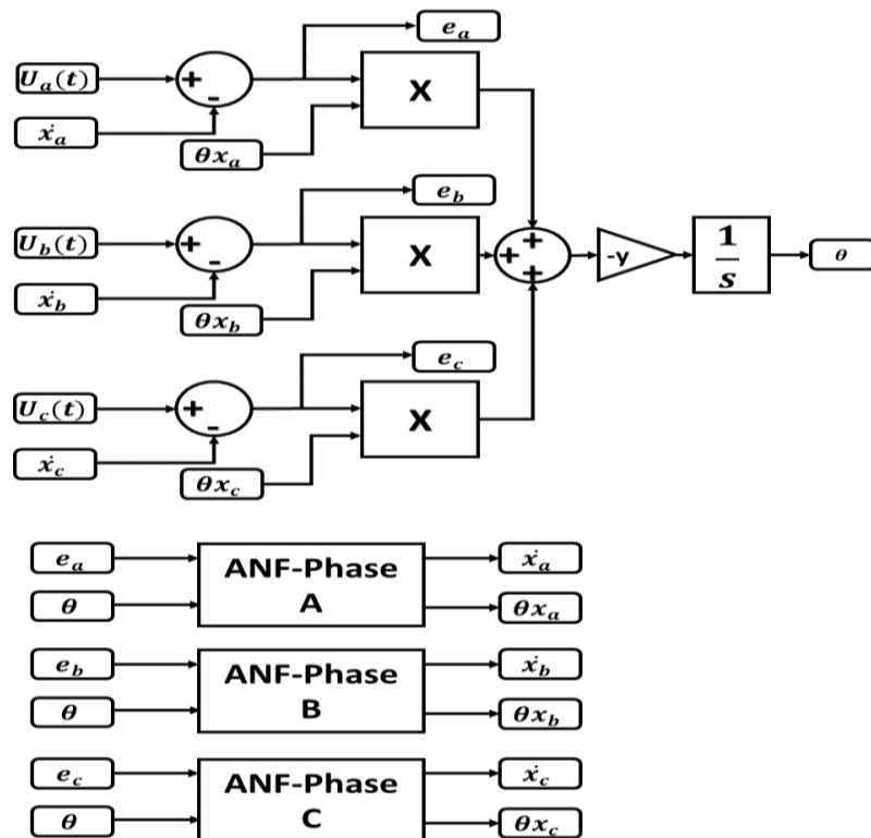
Figure 2. ANF structure for three-phase system
